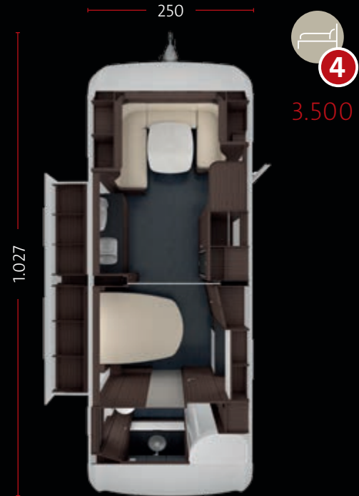
CELLINI 750 HTD 2,5 Slide-Out
